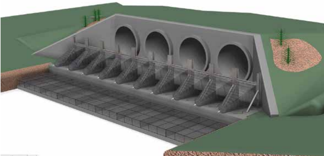
Figure 3 – Typical end-of-line application for the Ecosol™ Trash Rack.
